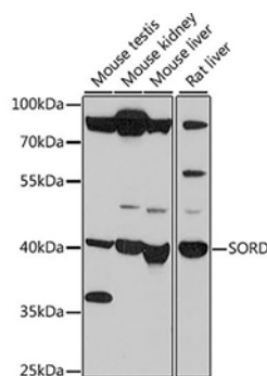
Fig. 1. Western blot analysis of extracts of various cell lines, using SORD antibody at 1:500 dilution.
